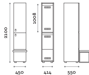
ANB12-23 Singola colonna 2 ante per panca Single column 2-tiers locker, bench version
