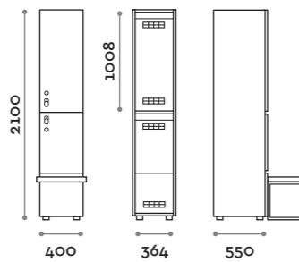
VANB35-23 Singola colonna 2 ante per panca Single column 2-tiers locker, bench version
