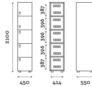
ANB05-23 Singola colonna 5 ante Single column 5-tiers locker
