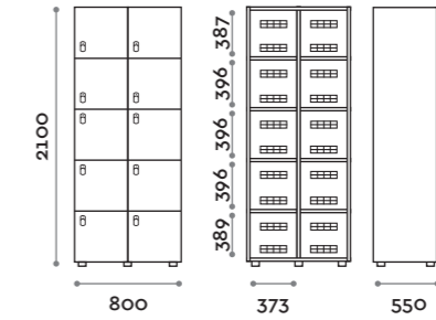
TANB4210-23 Doppia colonna 10 ante Double column 5-tiers locker 10 doors
