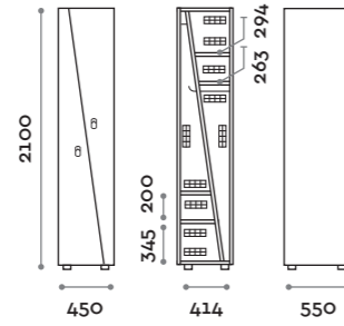
ATRO2-23 Singola colonna 2 ante trapezoidali Single column locker with 2 trapezoidal doors
